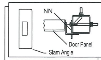
(Option Padlock Arrangement ) APLAR
